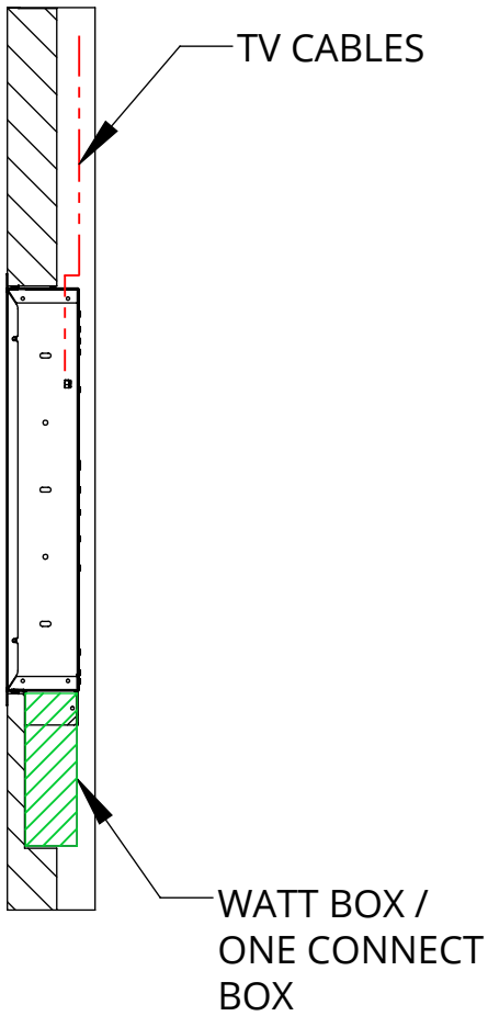
SECTION VIEW
