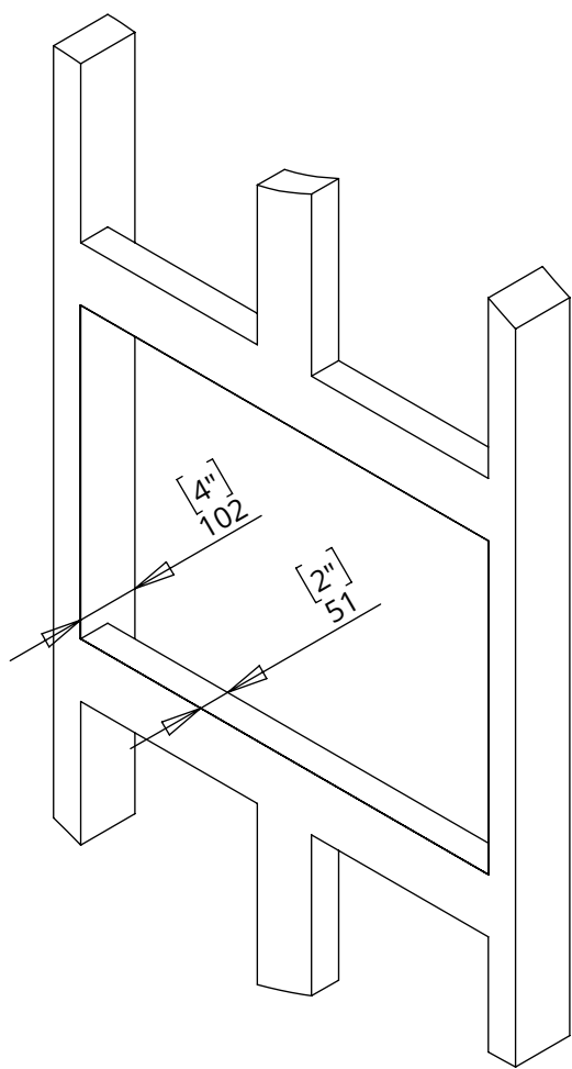
WALL STUDDING
