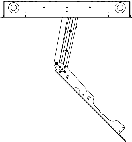
PSE90 OUT 45 - CLOCKWISE
