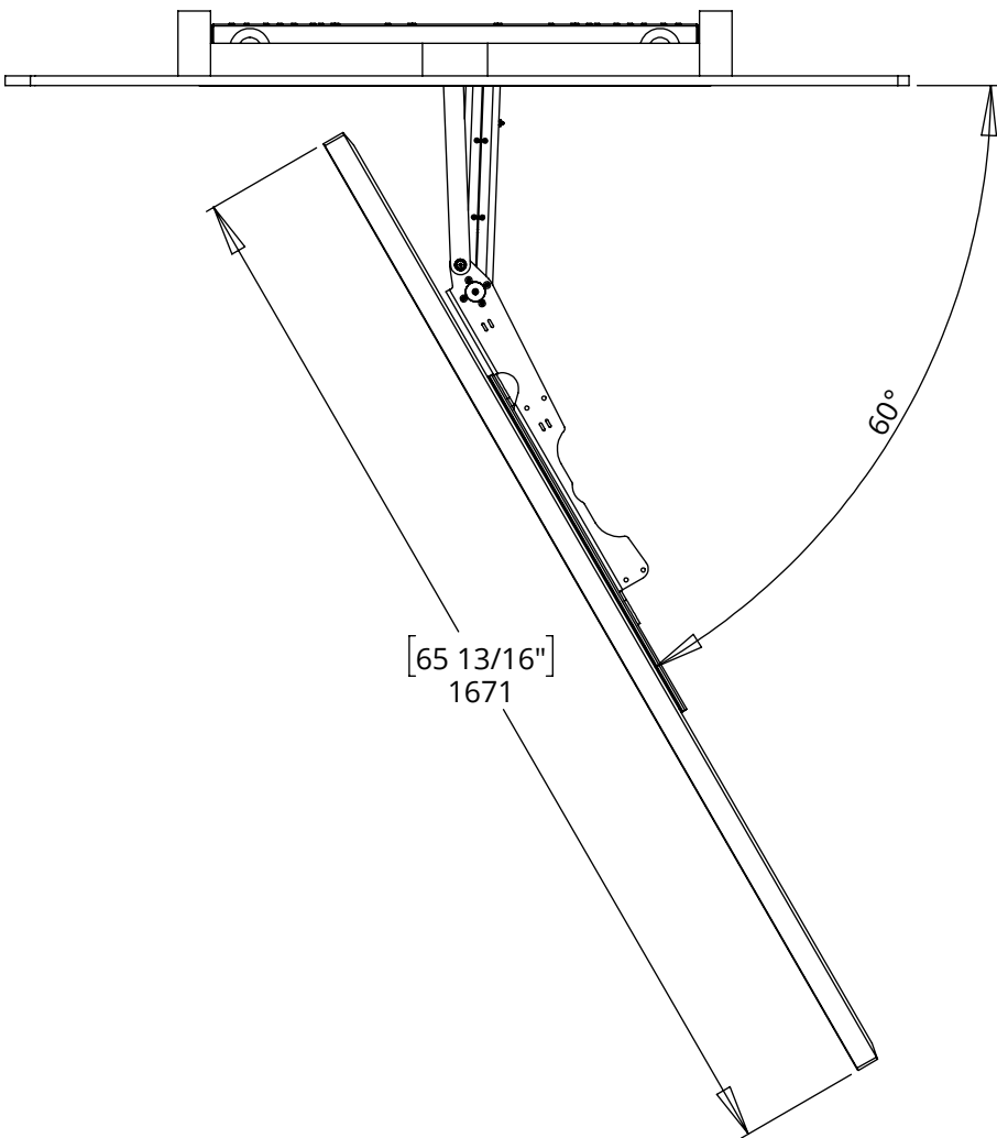
60 DEGREES - WITH OFFSET PLATES
