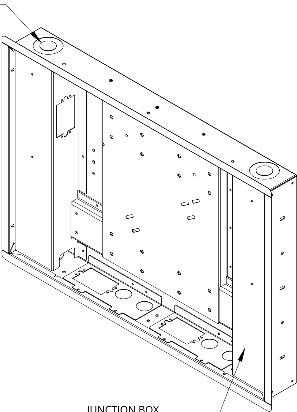
JUNCTION BOX KNOCK OUT ON INSIDE FACE OF PANEL
