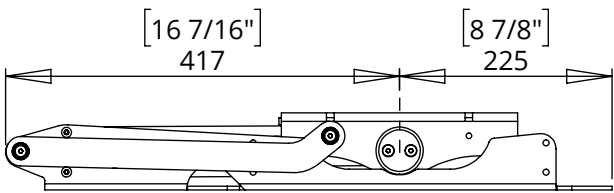
PSE90-CW Top View
