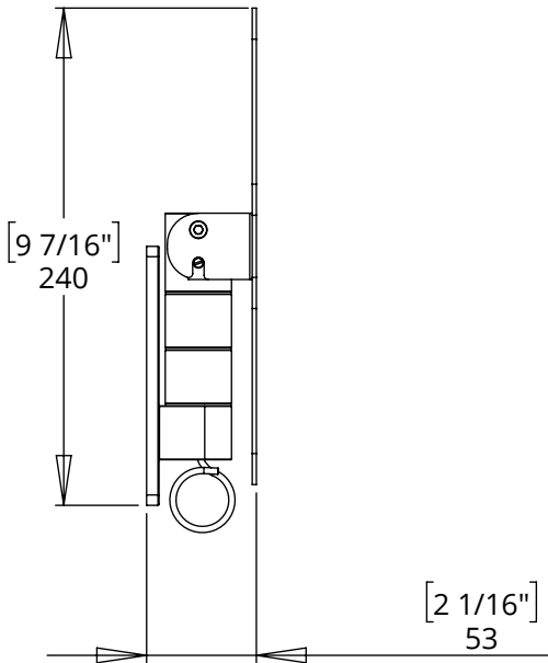
SIDE - CLOSED
